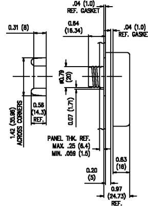
ENCLOSURE DRILLING METHOD BREATHER VENT
