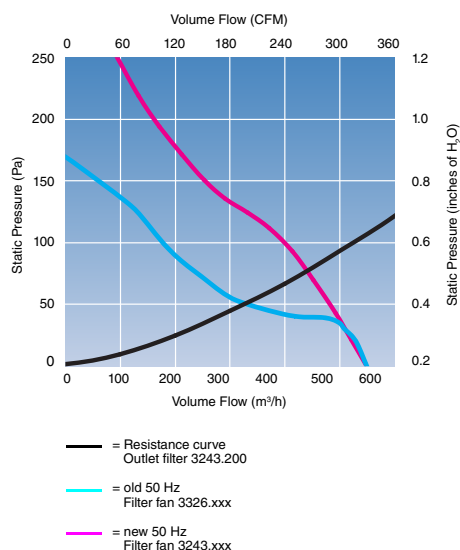
Performance chart — new vs. old filter fan design
