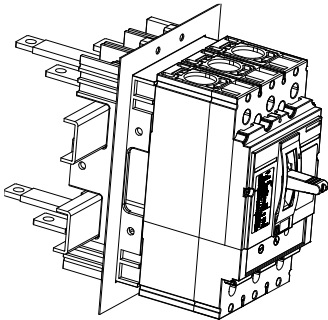
PIA22N Plug-In Base for M2 Unit: in [mm]
