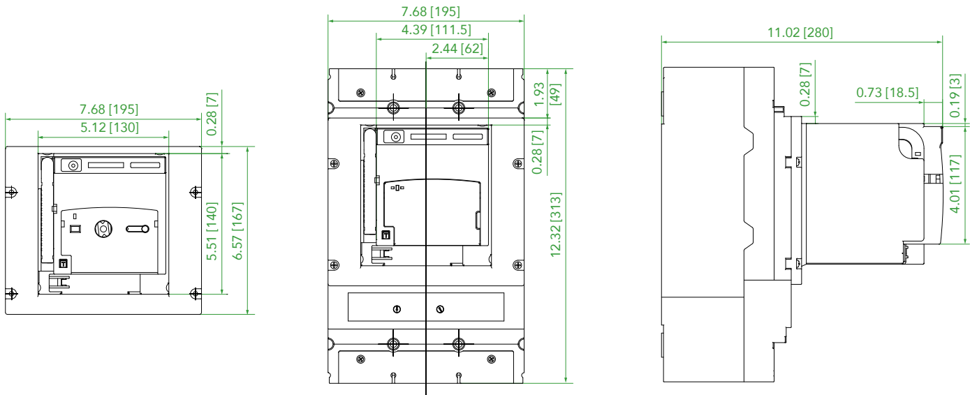
MOD24N Motor Operator for M4 Unit: in [mm]
