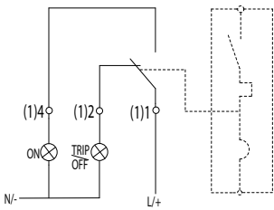
Wiring Diagram of Auxiliary Contact
