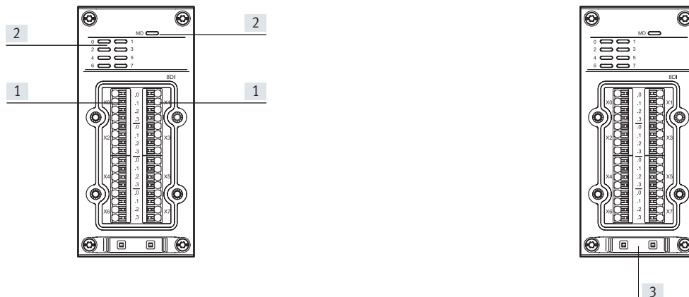
[1] Electrical connection, inputs [2] LED indicators [3] Space for inscription label
